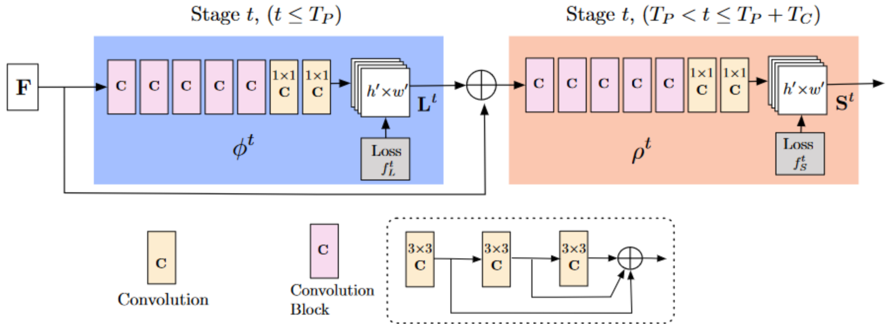
Fig. 3: Architecture of the multi-stage CNN. The first set
